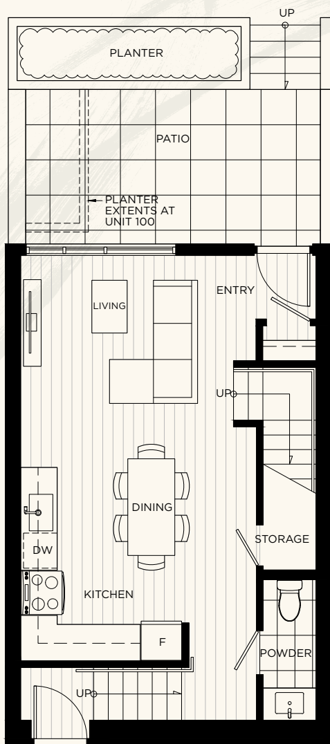
LEVEL 1
